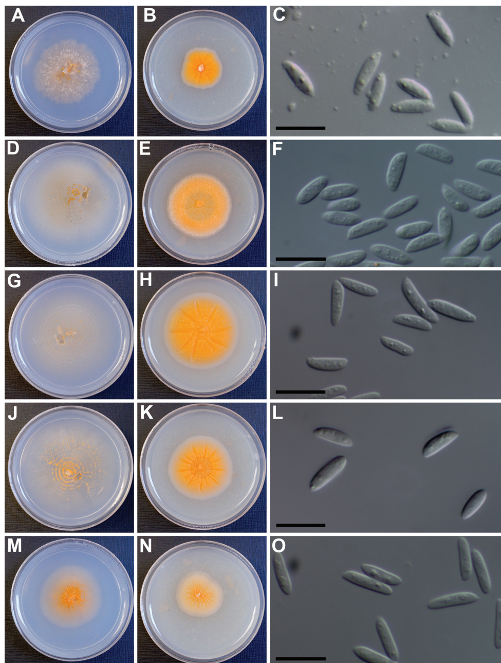
Figure 2. Lectera species. A–L L. colletotrichoides A–C IMI 166394 D–F , IMI 265740 G–I IMI 303685 J–L IMI 368065 M–O L. longa (IMI 181698) A, D, G, J, M colonies on PCA agar after 7 d B, E, H, K, N colonies on PDA agar after 7 d C, F, I, L, O : conidia mounted in lactic acid: bar = 10 µm.
